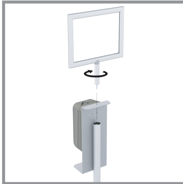
4. With optional frame - secure to the top of the pole as shown
